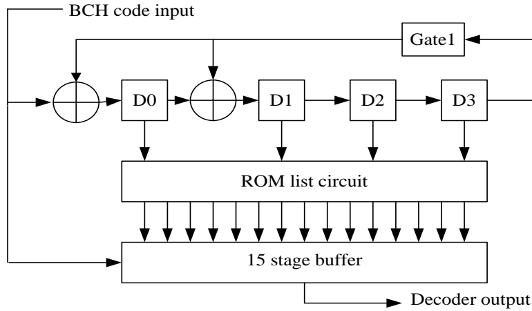
Figure 5-4 BCH(15,11,1) decoding logic
