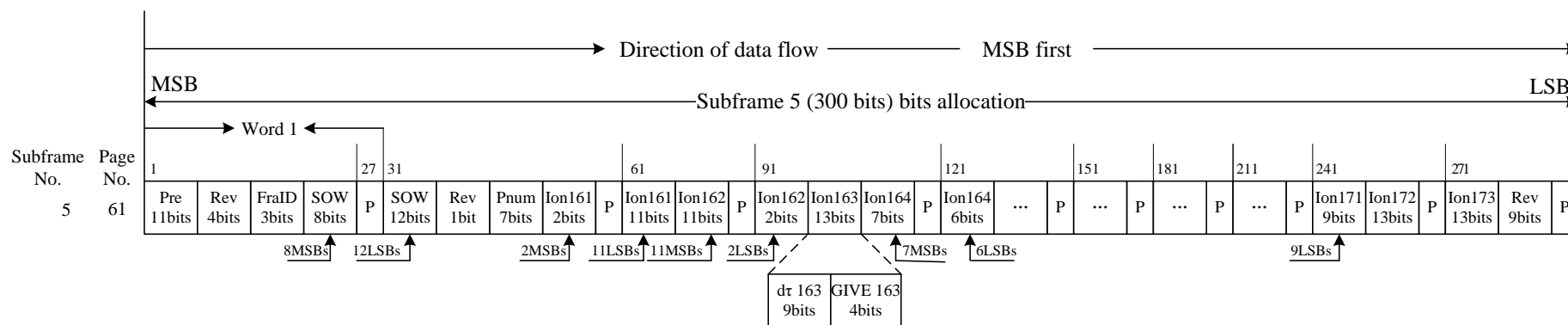
Figure 5-18-2 Bit allocation for page 61 of subframe 5 in format D2
