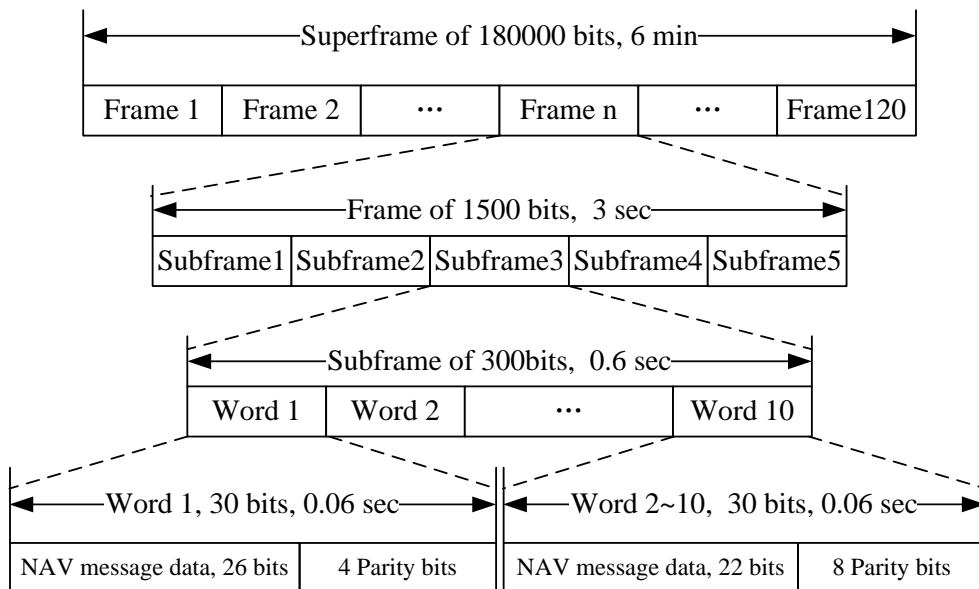
Figure 5-12 Structure of navigation message in format D2
