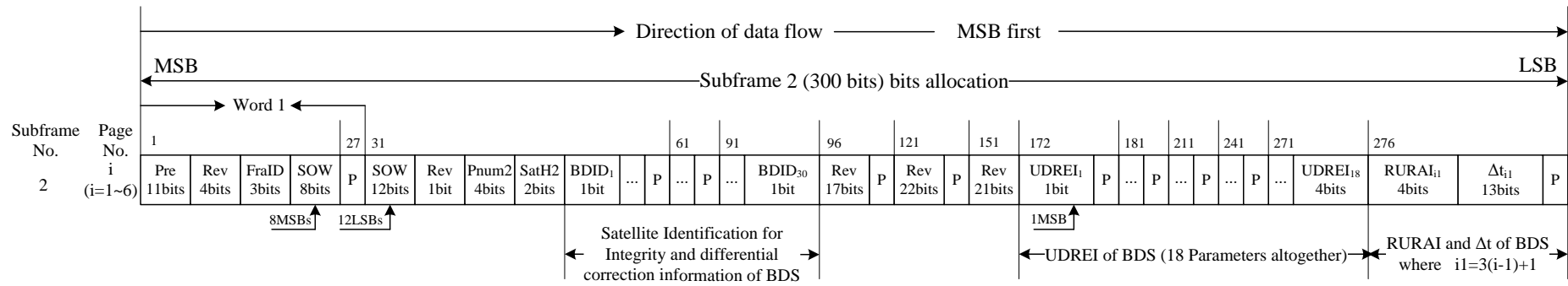
Figure 5-15 Bit allocation for subframe 2 in format D2
