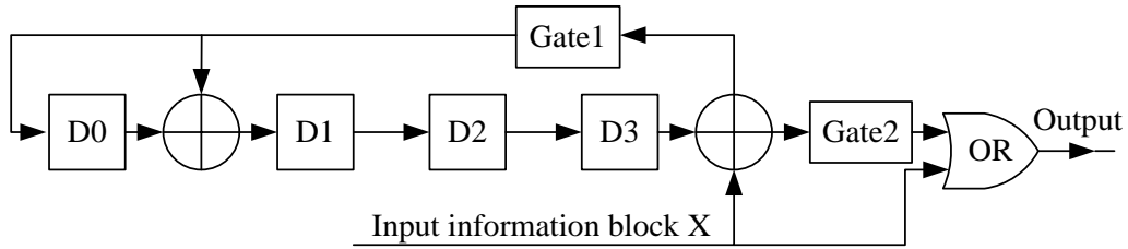
Figure 5-2 BCH(15, 11, 1) encoder
