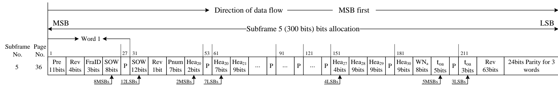
Figure 5-18-28 Bit allocation for page 36 of subframe 5 in format D2
