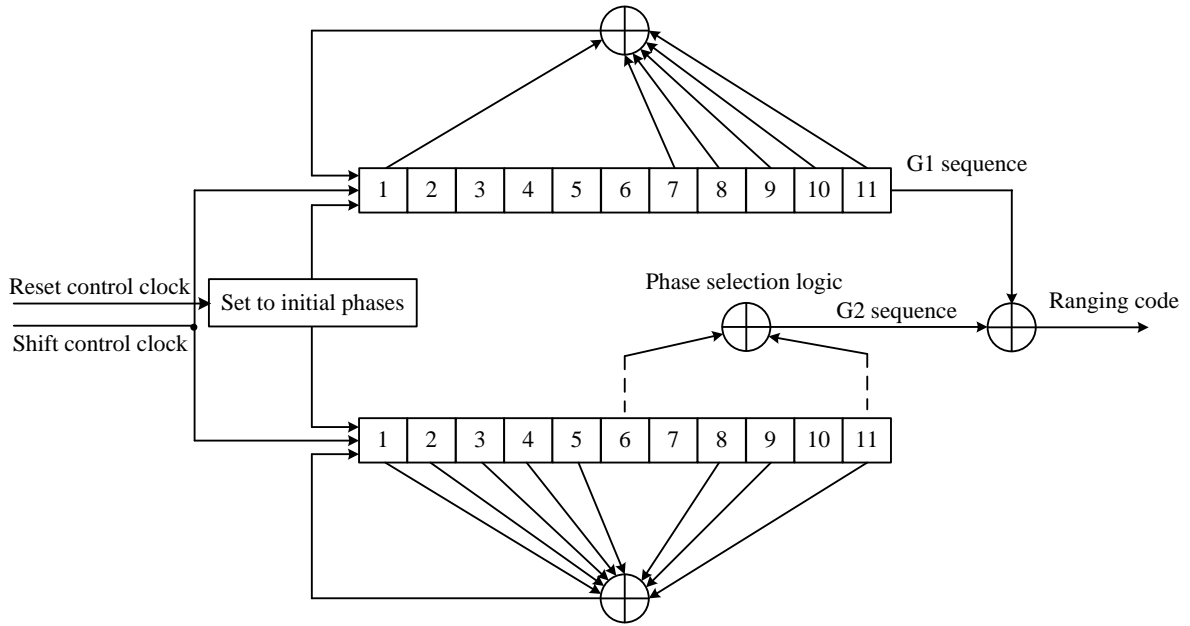
Figure 4-1 The generator of C_{B11}
