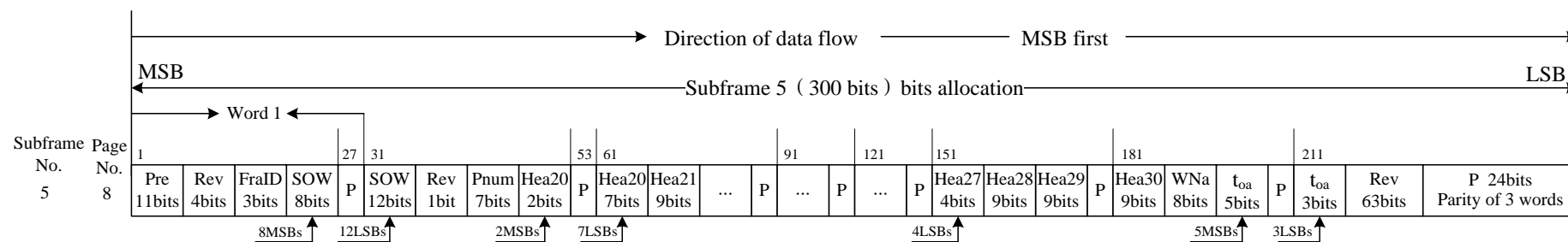
Figure 5-11-3 Bit allocation for page 8 of subframe 5 in format D1
